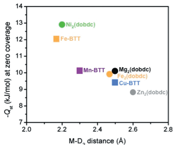
Fig. 3 Isosteric heats ( -Q_{\text{st}} ) plotted as a function of \text{M} – \text{D}_2 distances for two metal–organic framework families including \text{M}_2(\text{dobdc}) 6,18 and \text{M} – \text{BTT} . 5d,e,10c
