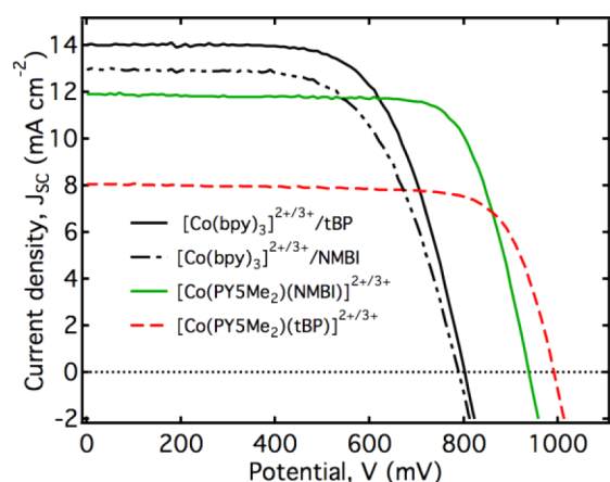
Figure 4. Comparison of DSC performance for optimized devices sensitized with MK2 based on 3a/3b (green line), 2a/2b (red dashed), [Co(bpy) 3 ] 2+/3+ /tBP (black solid), and [Co(bpy) 3 ] 2+/3+ /NMBI (black dotted) electrolytes in acetonitrile. IV characteristics are summarized in Table 3.
