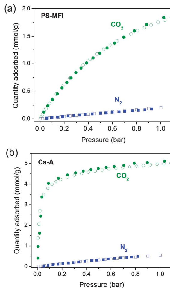
Fig. 1 Pure component CO 2 (green circles) and N 2 (blue squares) gas adsorption isotherms for (a) PS-MFI and (b) Ca-A, as measured at 25 °C using the high-throughput gas adsorption analyzer (solid symbols) and, for comparison, a Micromeritics ASAP® 2020 gas adsorption analyzer (open symbols).
