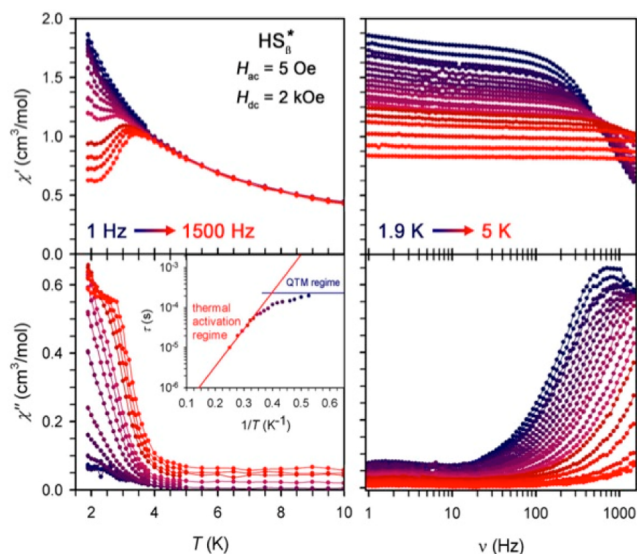
Figure 2. Temperature (left) and frequency (right) dependence of the in-phase ( \chi' , top) and out-of-phase ( \chi'' , bottom) components of the ac magnetic susceptibility data for HS \beta * at oscillating frequencies between 1 and 1500 Hz and temperatures between 1.9 and 5 K. Measurements were performed with a 5-Oe ac field and a 2000-Oe dc field. The solid lines are guides for the eye. Inset: Arrhenius plot showing the dependence of the magnetization relaxation time \tau upon inverse temperature, as obtained from the \chi'' versus \nu data. The solid red line corresponds to a linear fit to the data above 3 K, where relaxation can occur via a thermally activated process. At lower temperatures, relaxation becomes dominated by quantum tunneling of the magnetization (QTM).
