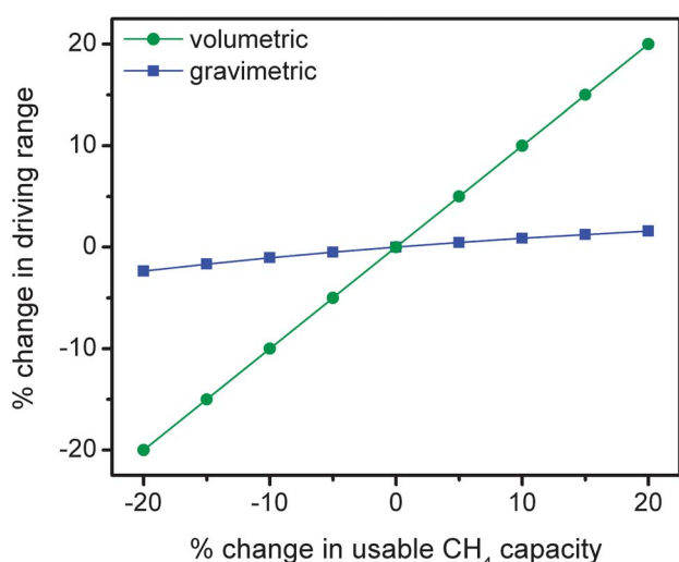
Fig. 8 Effects of changes in gravimetric and volumetric CH 4 usable capacity on vehicle driving range. To isolate each effect, the gravimetric case assumes a 10 GGE vehicle with a constant volumetric capacity, while the volumetric case assumes a fixed amount of space available for a fuel tank and a constant gravimetric capacity.
