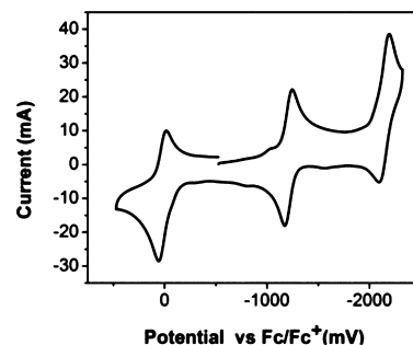
Figure 2. Cyclic voltammogram of 2 . Conditions: [ 2 ] = 1 mM, [NBu 4 PF 6 ] = 100 mM, acetonitrile solvent, scan rate = 100 mV/s, and working/reference/auxiliary electrodes = glassy carbon/silver wire/platinum wire. The Fc/Fc + couple is shown at 0 mV.
