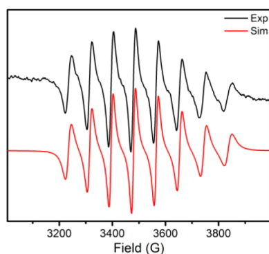
Figure 1. Room temperature X-band EPR spectrum of 2 in 99:1 CH 2 Cl 2 /CH 3 CN (black, top) and simulated spectrum [ g = 1.9745 , A(V^{51}, I=7/2) = 79.2 \times 10^{-4} \text{ cm}^{-1} ] (red, bottom).
