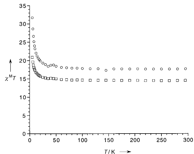
Figure 4. Magnetic behavior of 1 (□) and 2 (○) in an applied field of 1 kG. The data collected at 10 kG for each sample are essentially superimposable. \chi^M T in \text{cm}^3 \text{K mol}^{-1} .
