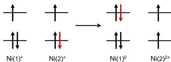
Figure 7. Schematic illustration of the excited states in 1' (right) found from CASSCF calculations using an extended active space. The excited state features a Ni 2+ center with a parallel alignment of spins according to Hund's rule. The itinerant electron is highlighted in red.
