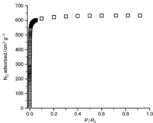
Figure 3. Isotherm for the adsorption of \text{N}_2 within 2d at 77 K.
